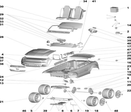
45 - SEAT BELT NOT SHOWN
