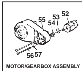
ASSEMBLY A
